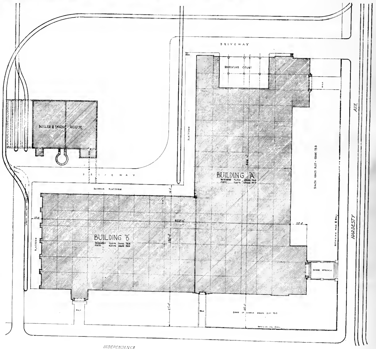
PLOT PLAN
